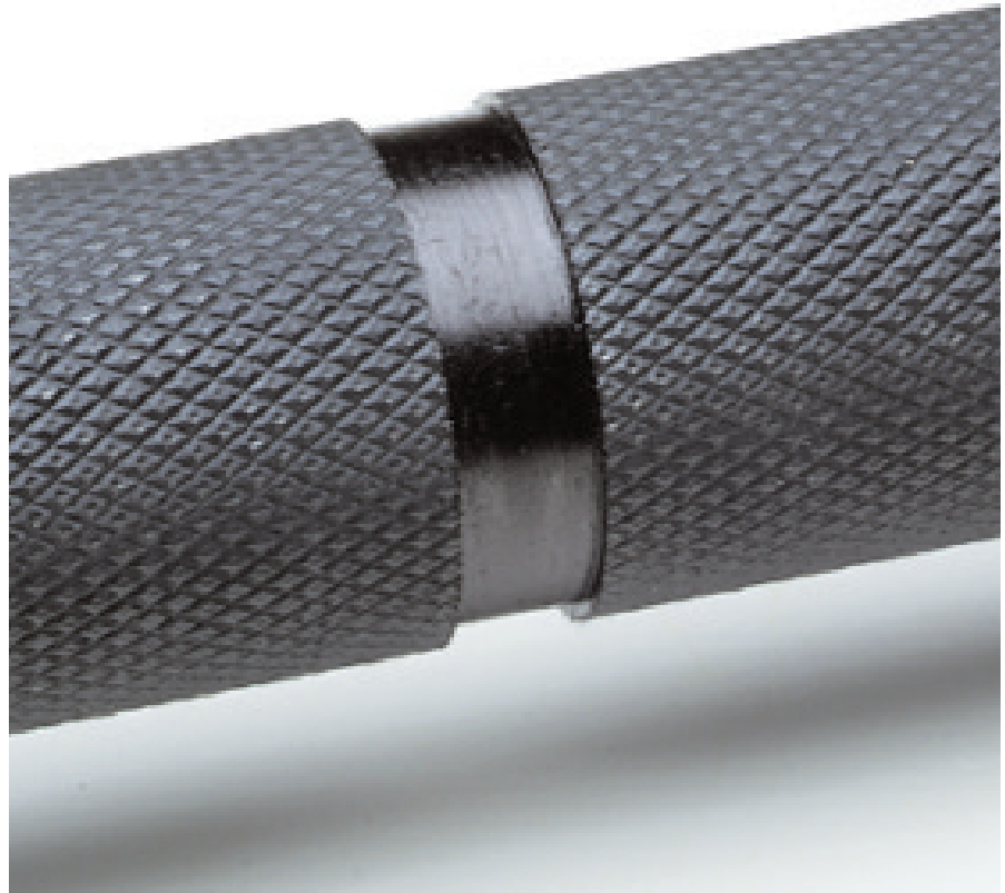
A bar showing a typical “suicide groove”. This cosmetic feature will weaken the bar at this point, and is often the precursor of bar failure.
